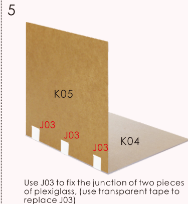
scale:1:10 K05 plexiglass(transparent) 20*20*0.15(2 pieces)
