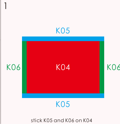
scale:1:10 K06 plexiglass(transparent) 20*17.7*0.15(2 pieces)
